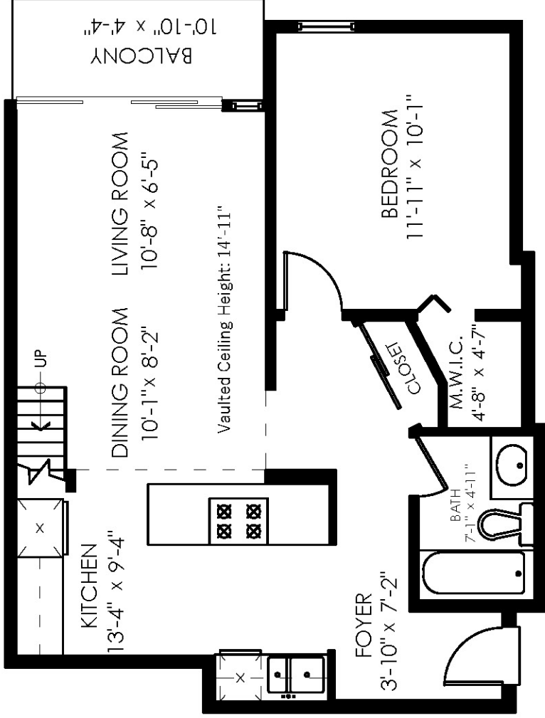
Main Floor: 618 Sq.Ft. Ceiling Height: 8'-0"
